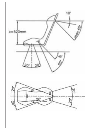
Drawing No. 253-42
