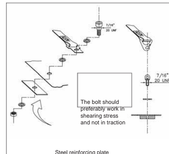
Steel reinforcing plate fixed to the car's chassis
